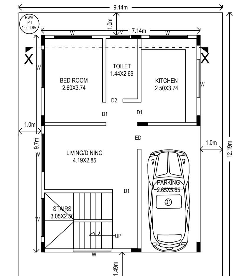
8.5 m wide ROAD GROUND FLOOR PLAN
