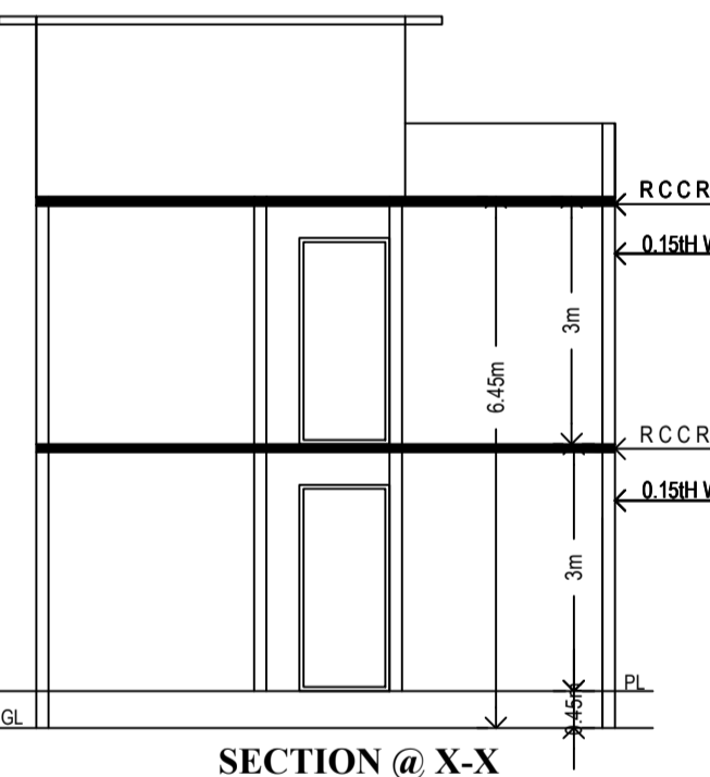
SECTION @ X-X
